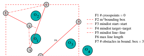
Fig. 5. Visualization of navigation task features that are used for classifying navigation tasks.
